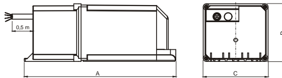
Fig.Y (600W-1000W)
